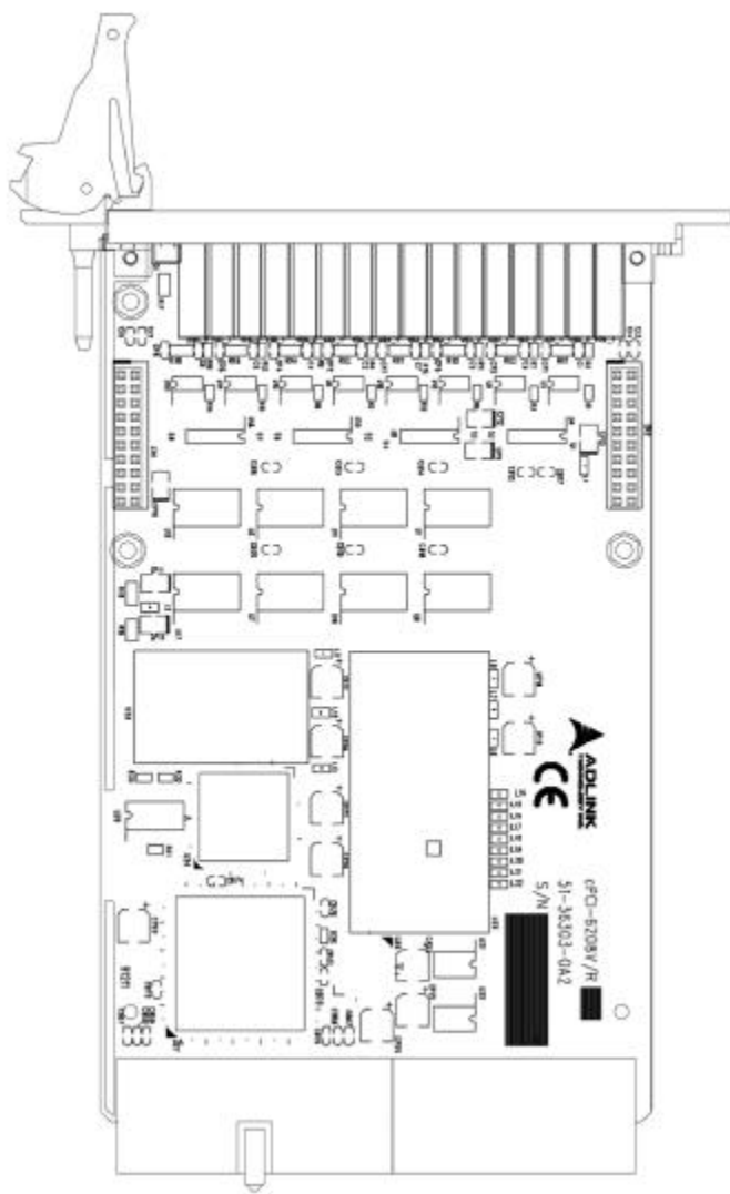
Figure 4: cPCI-6208V/R Layout
