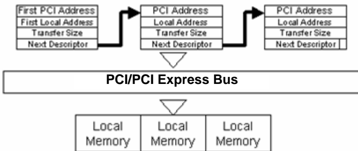
Figure 4-5: Scatter/gather DMA for digital output
