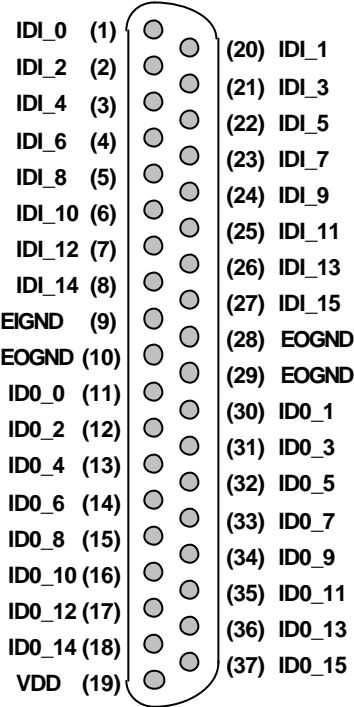
Figure 2.7 Pin assignment of Connector CN3
