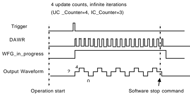
Figure 29: Stop mode II
