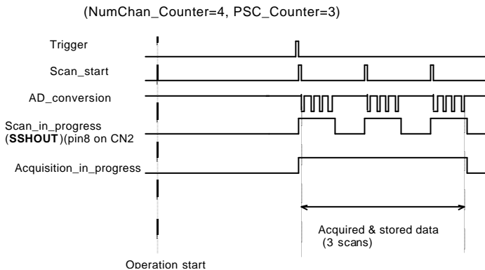
Figure 18: Post trigger
