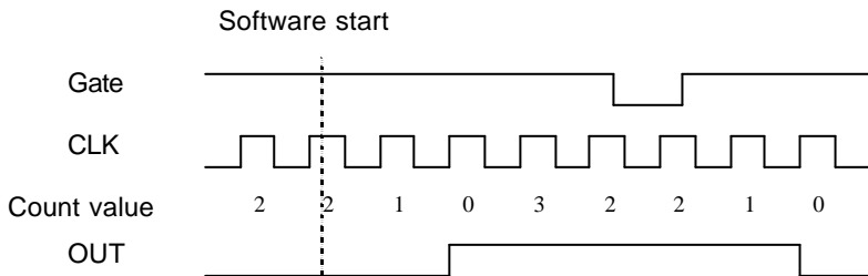
Figure 34: Mode 4 Operation
