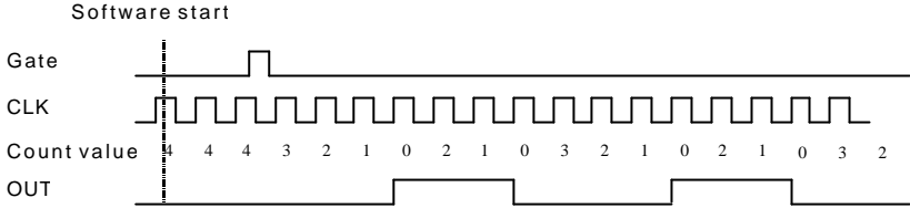
Figure 37: Mode 7 Operation
