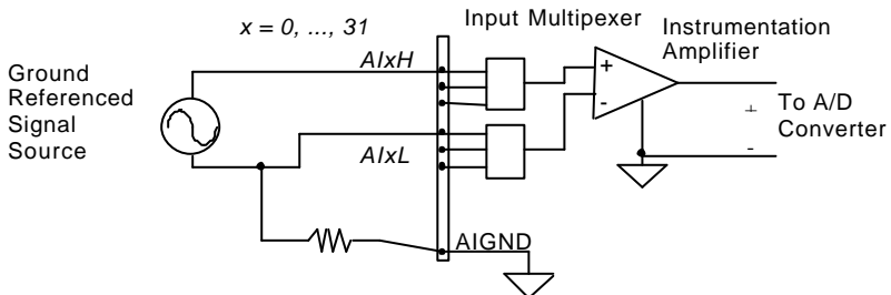
Figure 8: Floating source and differential input
