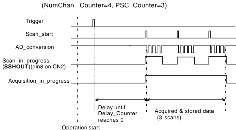
Figure 19: Delay trigger
