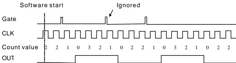
Figure 36: Mode 6 Operation
