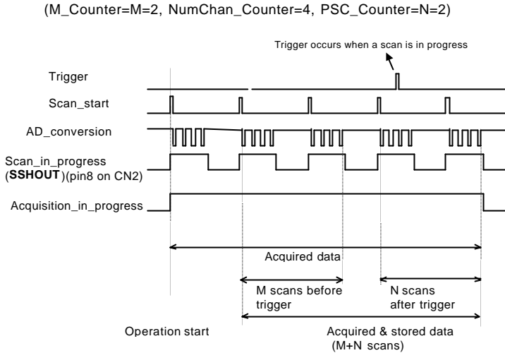
Figure 17: Middle trigger (trigger occurs when a scan is in progress)
