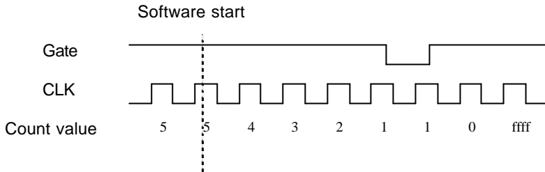
Figure 31: Mode 1 Operation
