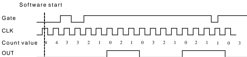
Figure 38: Mode 8 Operation
