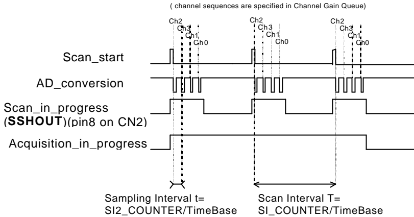
Figure 11: Scan Timing
