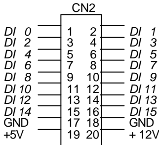
Figure 3.1. Pin Assignment of CN2
