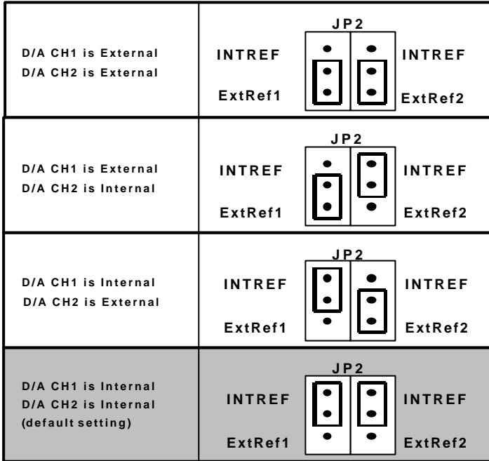
Figure 2.8 D/A Voltage Setting
