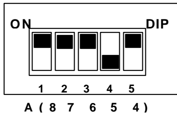
Figure 2.2 Default Base Address Setting
