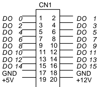
Figure 3.2. Pin Assignment of CN1
