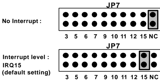
Figure 2.7 IRQ Level Setting
