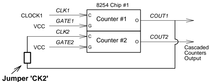
Figure 2.11 Example of 'user configurable cascaded counters'
