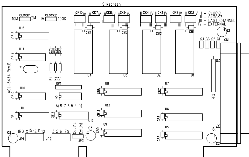
Figure 2.1 PCB Layout of the ACL-8454
