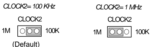
Figure 2.6 Jumper setting of CLOCK2
