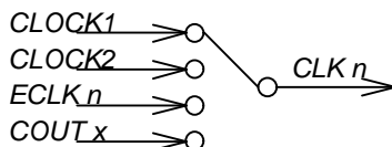
Figure 2.12 Clock Source of Counter #n
