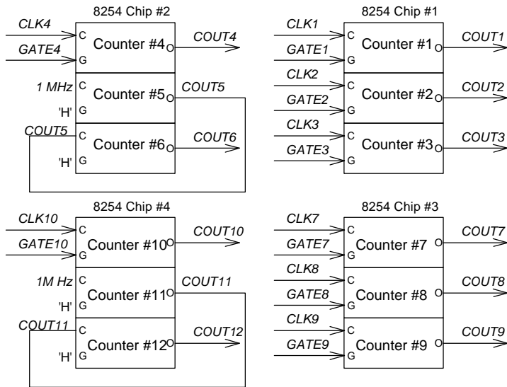
Figure 2.8 Counters Architectural
