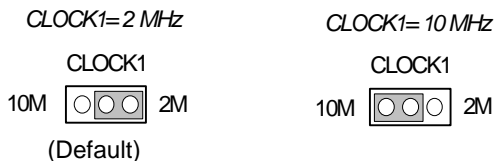
Figure 2.5 Jumper setting of CLOCK1
