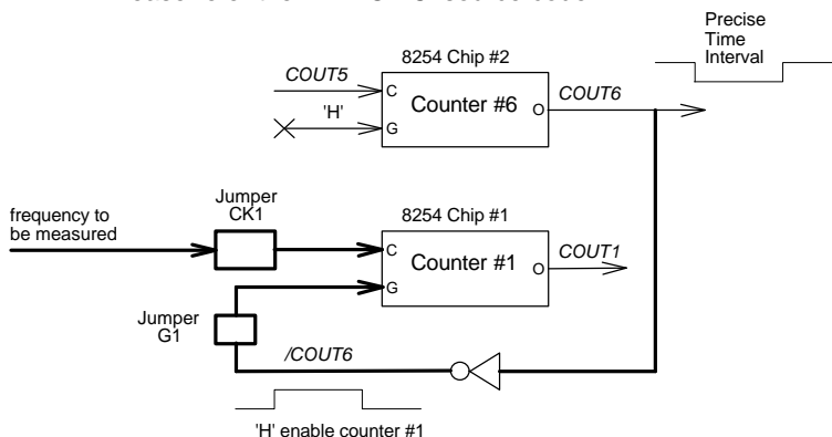
Figure 4.4 Example of frequency measurement (1)
