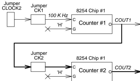
Figure 4.2.2 Example of frequency generator (2)
