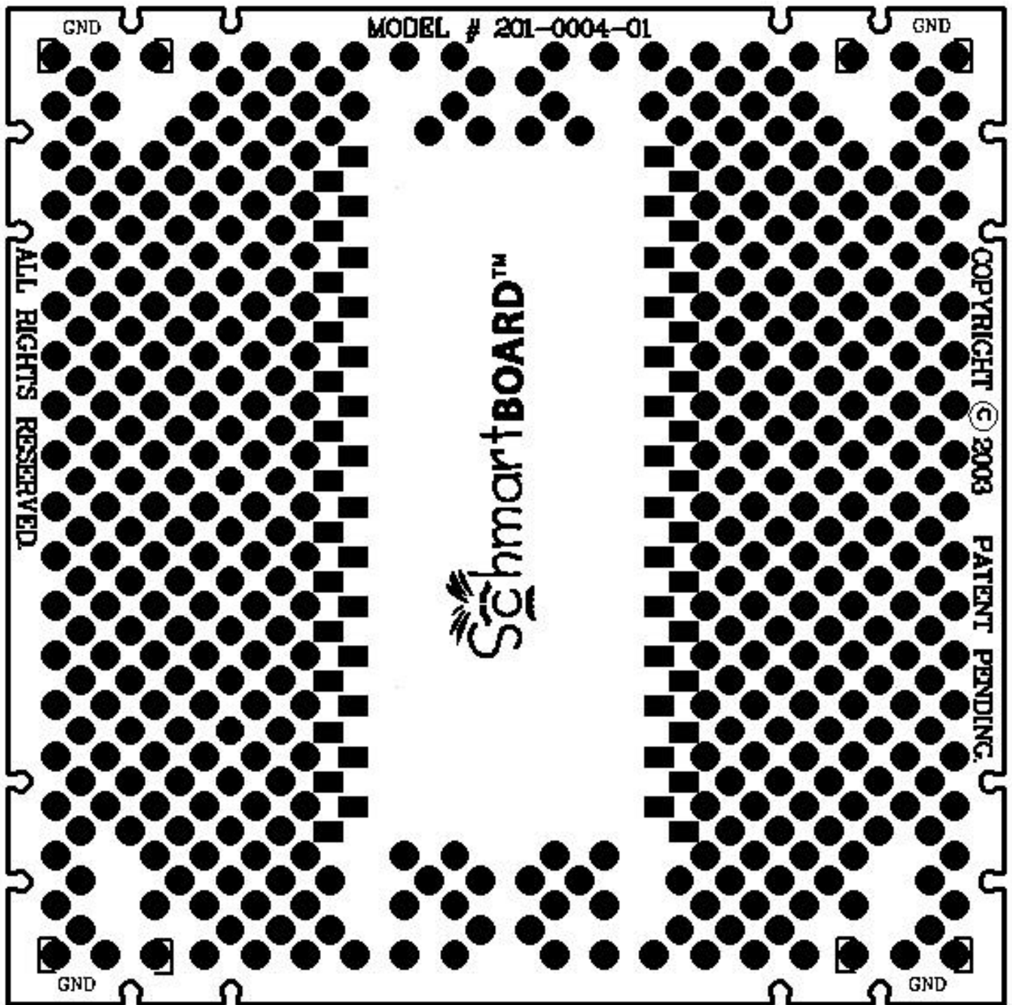
SO 4 –56 PINS (201-0004-01) Bottom Side
